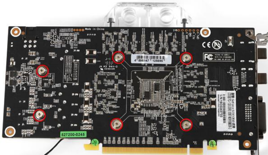
Attention to red position screw for installation drawing
